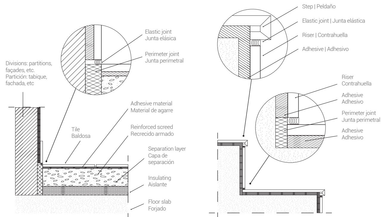
Detail of perimeter joint with sealant | Detalle de junta perimetral con sellante (UNE 138002:2017)
